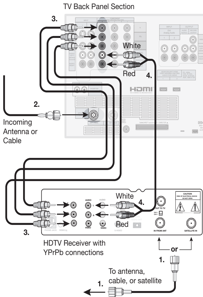
Figure 11. Connecting an External HDTV Receiver with Component Video Connections
