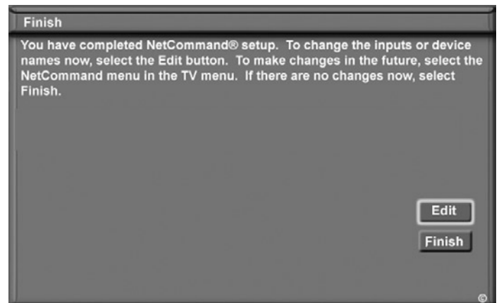
Figure 27. Finish screen
