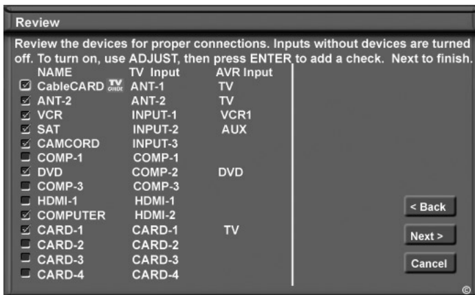
Figure 6. Review screen
