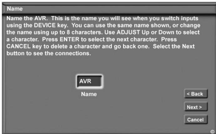
Figure 12. Name screen
