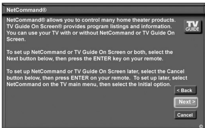
Figure 2. Information screen
