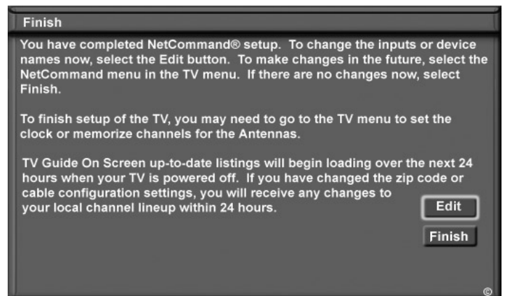
Figure 7. Finish screen
