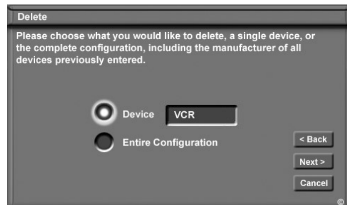
Figure 26. Delete screen
