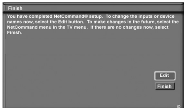
Figure 14. Finish screen
